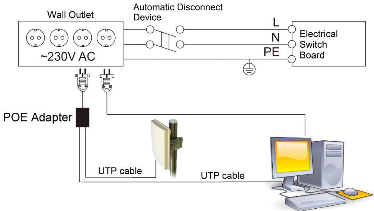
1 Figure: Building installation scheme
