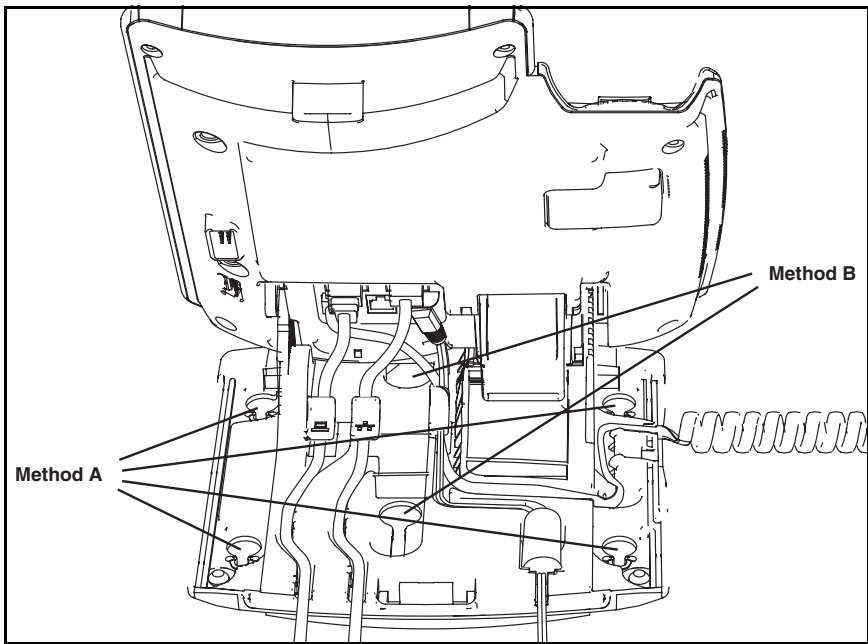
Figure 6: Cable routing tracks and mounting holes
