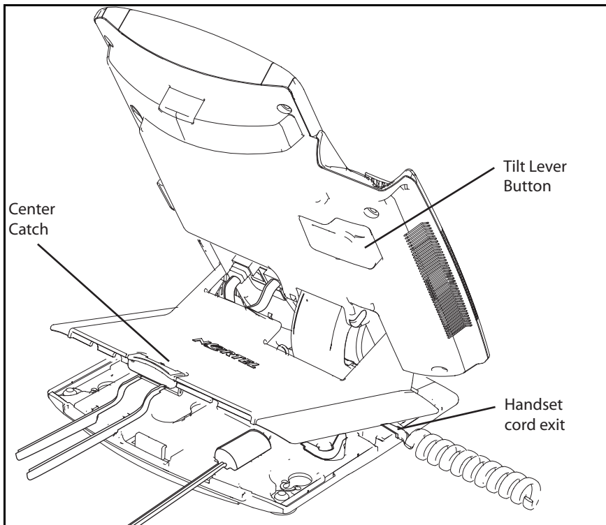
Figure 5: Remove the stand cover
